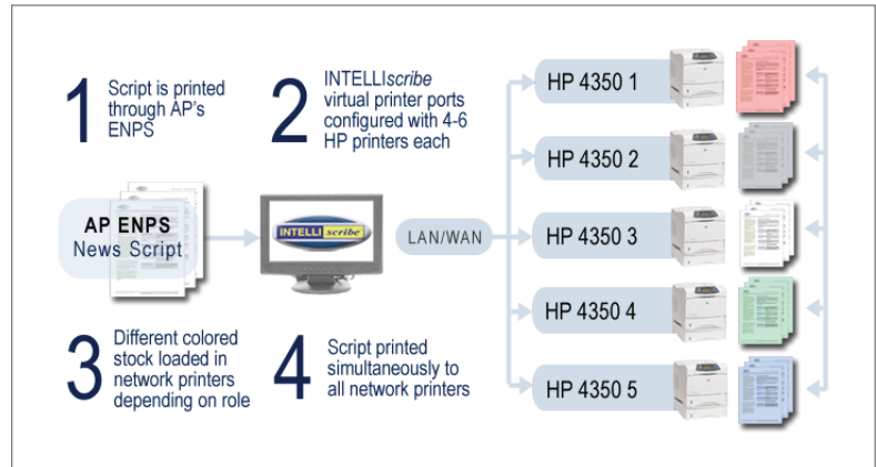
Newsroom script printing setup with INTELLscribe installed on a server
