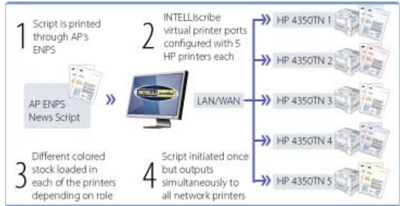
Newsroom script printing setup with INTELLiscribe installed on a server
